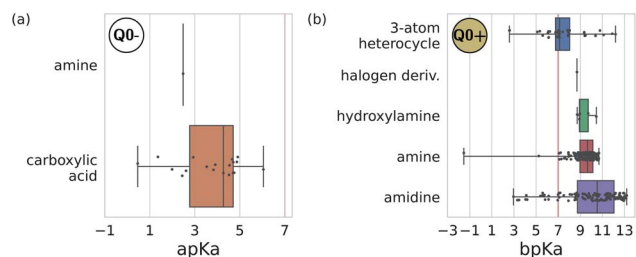
Fig. 7 Predominant functional groups mapped to the charged bead type Q0± within our 5 + 1 reduced Martini model. 25,35 (a) Functional groups with apKa ≤ 7 are most likely to be negatively charged under physiological conditions (pH \approx 7.3) and are mapped to the Q0- bead. (b) Those with bpKa ≥ 7 are most likely to be positively charged and are mapped to the Q0+ bead.
