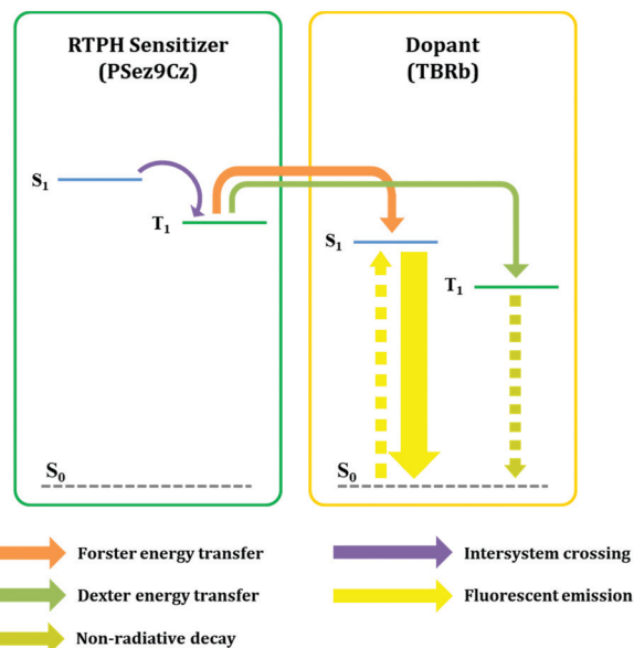
Fig. 3 Scheme of the energy transfer process in the RTPH sensitized fluorescent EML.
