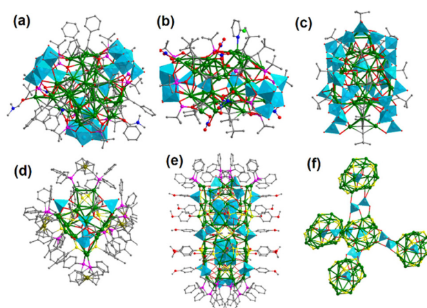
Fig. 18 Molecular structures of (a) [(\text{O}_2)\text{V}_2\text{O}_6]_3@[\text{Ag}_{43}@[(\text{BuPO}_3)_4\text{V}_4\text{O}_8]_3] , (b) [(\text{O}_2)\text{V}_2\text{O}_6]_2@[\text{Ag}_{36}@[(\text{BuPO}_3)_4\text{V}_4\text{O}_8]_2] , (c) (\text{V}_2\text{O}_7)_2@[\text{Ag}_{44}(\text{V}_{32}\text{O}_{96})] , (d) \text{MoO}_4@[\text{Ag}_{24}((\text{MoO}_4)_4)] and (e) (\text{MoO}_4)_5@[\text{Ag}_{52}((\text{MoO}_4)_{10})] . (f) Each \text{CrO}_4@[\text{Ag}_{20} \text{ subunit}] connected to its adjacent four neighbours by \text{Cr}_2\text{O}_7^{2-} . (g) Molecular structure (left) and cyclic voltammogram (right) of \text{SiW}_{10}\text{O}_{37}@[\text{Ag}_{41}-\beta\text{-SiW}_{12}\text{O}_{40}] .
