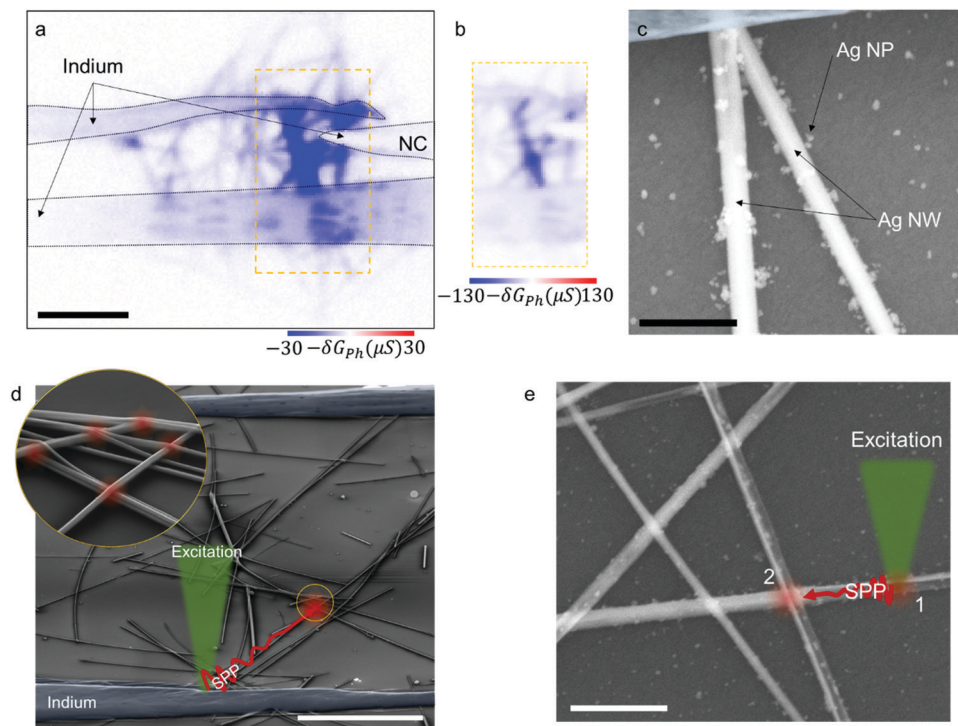
Fig. 4 (a) Photoconductive map of an Ag NP-decorated network device under a -100 mV bias. Outlines of the indium contacts are marked with black dashed lines. The needle on the right side marked with NC is an indium needle that was not connected to the device electrically. The map scale is saturated to reveal the photoconductive change over the Ag NWs outside of the device and over the indium needles. Maps were taken with a 532 nm laser at 93 \mu\text{W} . The scale bar is 10 \mu\text{m} . (b) Unsaturated -\delta G_{ph} map of the area marked with the yellow dashed rectangle in (a) and (c). Close-up SEM micrograph of Ag NWs decorated with Ag NPs. Indium contact is false-colored with blue. The scale bar is 500 \text{ nm} . (d) SPP-assisted bolometric response depicted in a false-colored SEM image. The excitation creates SPPs at the contacts or regions where the light coupling to the metal structure is possible. The SPPs travel to the NW–NW junctions and the local field enhancement creates hot spots. The scale bar is 20 \mu\text{m} . (e) A similar mechanism is depicted in the SEM image of Ag NP-decorated Ag NWs. The light coupling is possible near the nanowires thanks to the Ag NPs, which create two hot spots, marked with 1 and 2 on the SEM image. The scale bar is 1 \mu\text{m} .
