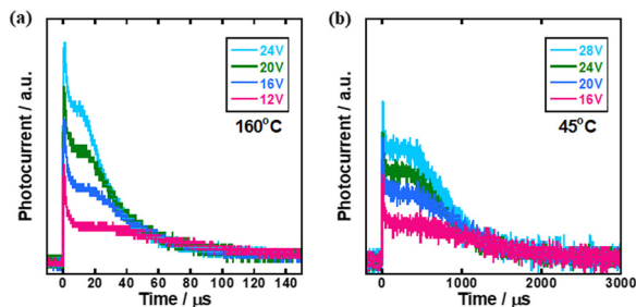
Fig. 6 Transient photocurrent curves for holes (a) in the N* phase of the mixture of compounds 1–3 at 160 °C and (b) in the glassy N* phase at 45 °C. The sample thickness was 4 \mu\text{m} and the wavelength of excitation light was 356 nm.
