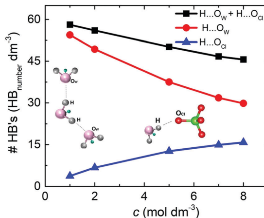
Fig. 4 Density of hydrogen bonds (HB's) as a function of the \text{NaClO}_4 molar concentration. The blue curve stands for \text{H}\cdots\text{OCl} pairs ( \blacktriangle ), the red curve for \text{H}\cdots\text{O}_w pairs ( \bullet ), and the black curve ( \blacksquare ) is the sum of both pairs.
