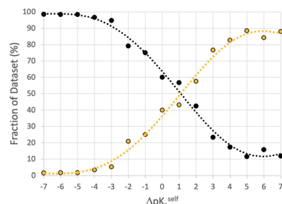
Fig. 9 Relative occurrence (%) of non-zwitterions (black) versus zwitterions (orange) as a function of \Delta pK_{a,\text{self}} (bins of one \Delta pK_a unit). Data for unsolvated forms (a) are compared to hydrates (b). Dataset-2 is filtered according to: only one main component, no Q4 zwitterions.
