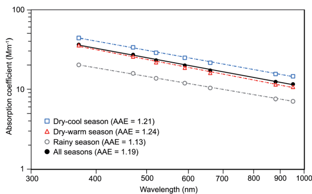
Fig. 1 Power law distributions of absorption coefficients for the 370–950 nm wavelength range as measured by the Aethalometer AE33 for each climatological season of Mexico City and during the two-year study. The AAE values are the arithmetic means obtained from the linear regressions between the log-transformed hourly b_{\text{abs}} records and wavelength spectra, considering the full study period, and individual climatological seasons.
