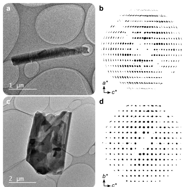
Fig. 2 (a) A crystal of \mathbf{1}_{\text{MeOH}} and (b) reconstructed reciprocal lattice based on the acquired 3DED data projected along b^* . (c) A crystal of \mathbf{2} and (d) reconstructed reciprocal lattice based on the 3DED data projected along a^* .
