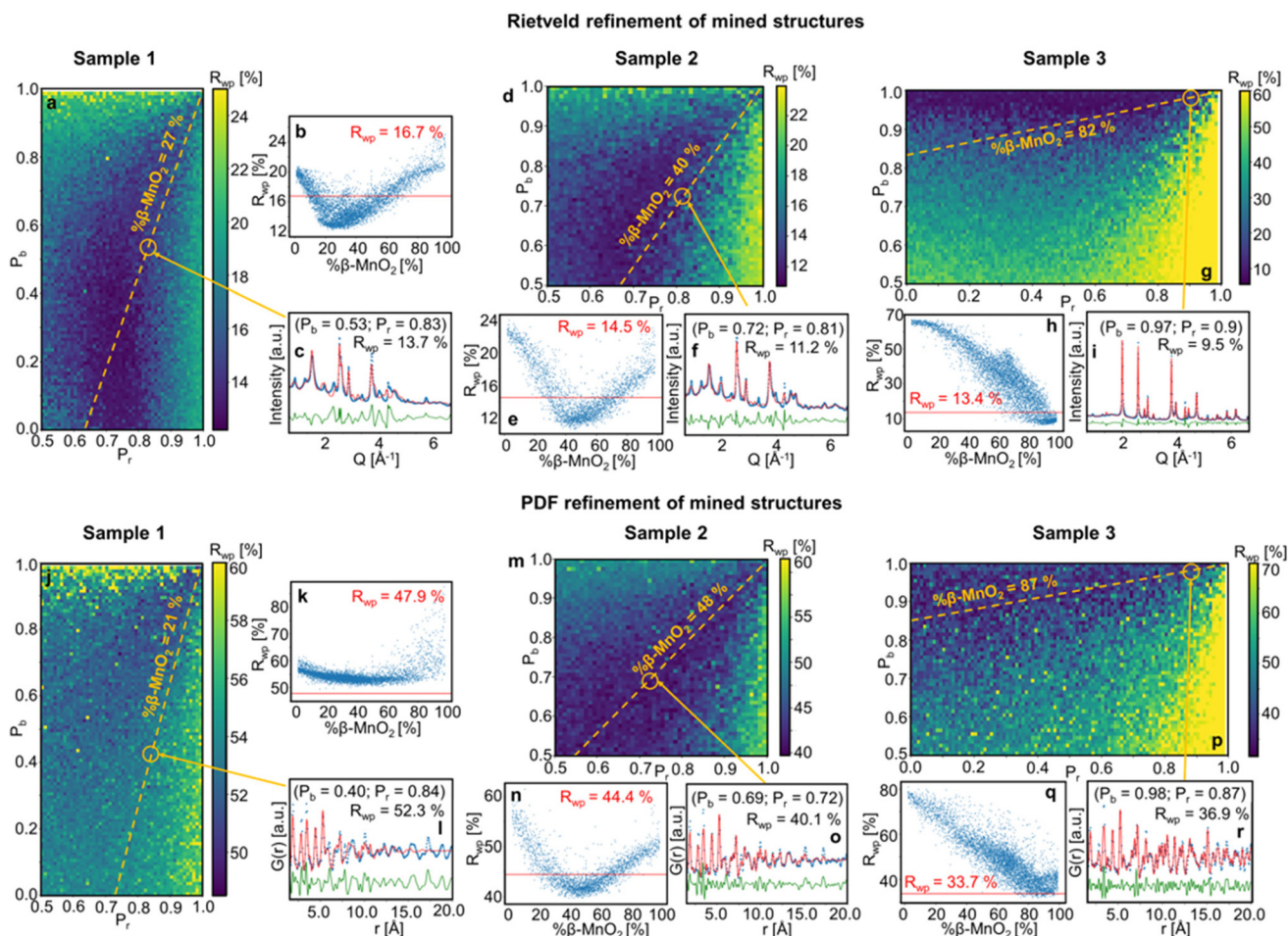
Fig. 6 Results from fitting of mined structures of sample 1, 2 and 3. Contour plots show R_{wp} values from Rietveld (a, d and g) and PDF refinements (j, m and p) as a function of (P_b, P_r) for each superstructure for samples 1, 2 and 3, respectively. The same R_{wp} values as a function of the \beta - MnO_2 fraction are shown in (b, e and h) and (k, n and q), respectively. The red solid line represents the R_{wp} value of the refinement of a two-phase mixture of parent structure \beta - and R - MnO_2 . The Rietveld and PDF refinement of the superstructure with (P_b, P_r) values determined from the peak-fitting analysis are shown in (c, f and h) and (l, o and r), respectively.
