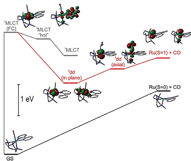
Fig. 9 Basic energy diagram representing the SOMOs of the states involved in the photophysics and photochemistry of RU18 . Taken from ref. 61. Copyright permission © 2020 American Chemical Society.
