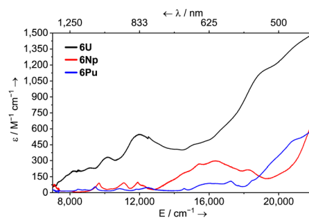
Fig. 2 UV-vis-NIR spectra of [\text{U}(\text{TMP})_2\text{Bn}_2\text{K}(\text{toluene})] ( 6U , black line) in THF (0.97 mM), and [\text{Np}(\text{TMP})_2\text{Bn}_2\text{K}(\text{toluene})] ( 6Np , red line) in toluene (0.50 mM), and [\text{Pu}(\text{TMP})_2\text{Bn}_2\text{K}(\text{toluene})] ( 6Pu , blue line) in toluene (1.00 mM) between 7000–22 000 \text{cm}^{-1} (1429–455 nm) at room temperature.
