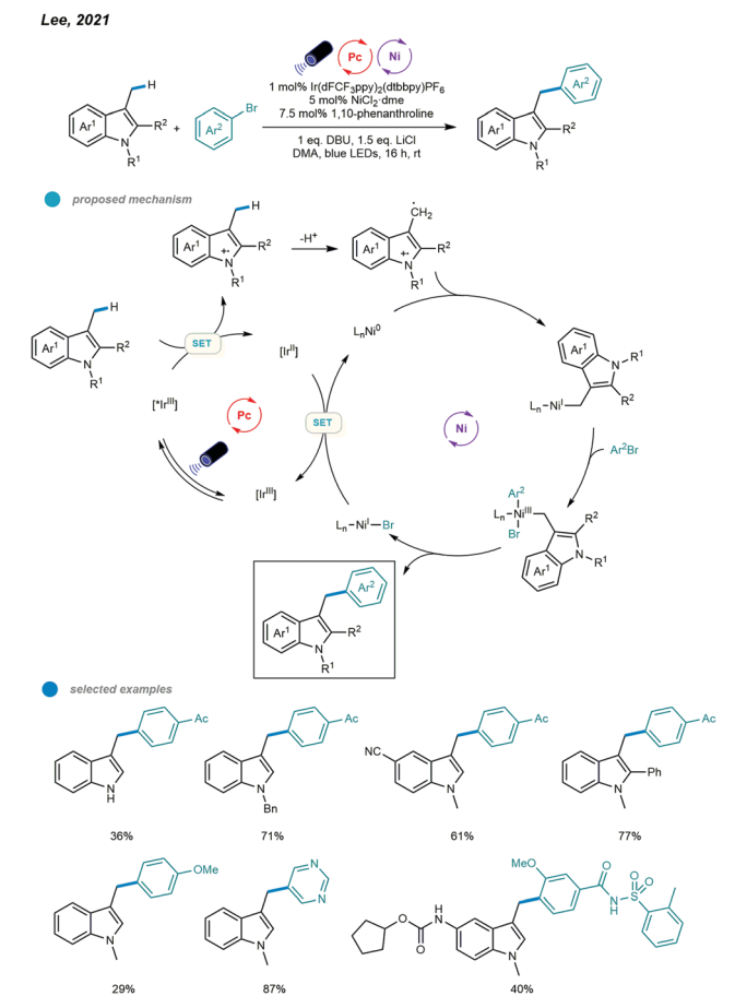
Scheme 6 Photoredox and nickel dual-catalyzed benzylic C(sp 3 )-H arylation of indole derivatives.
