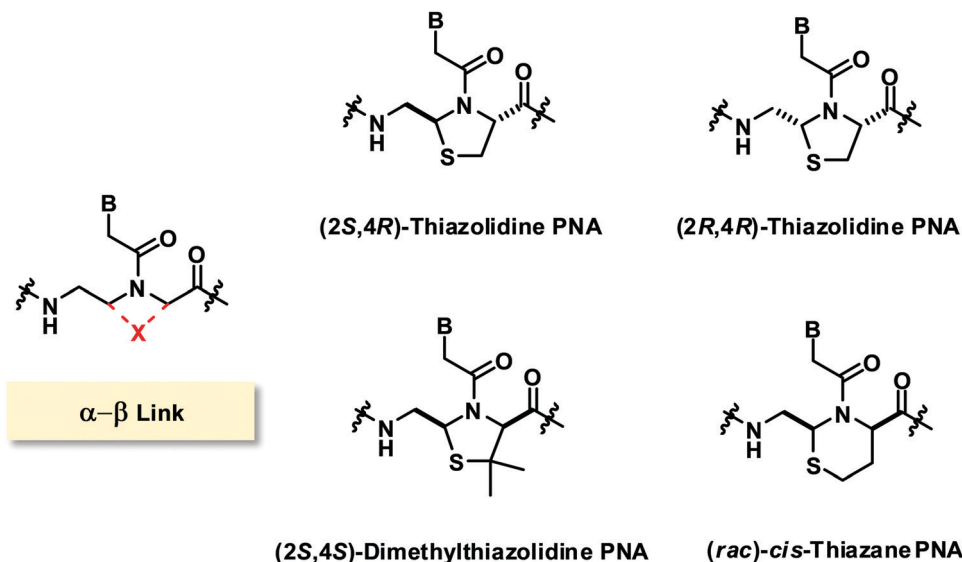
Fig. 23 Structures of modified PNA with (\alpha-\beta) -linkage.
