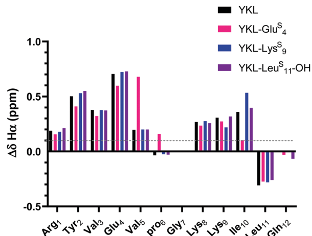
Fig. 3 \Delta\delta_{\text{H}\alpha} (test \delta_{\text{H}\alpha} - \text{unfolded control } \delta_{\text{H}\alpha} ) for YKL-Glu S 4 , YKL-Lys S 9 , and YKL-Leu S 11 -OH in comparison to YKL. Three consecutive \Delta\delta_{\text{H}\alpha} values of greater than 0.1 ppm (shown in figure) is indicative of \beta -sheet structure. Besides slight variations around where the thioamide is incorporated, the \Delta\delta_{\text{H}\alpha} values are like YKL for all positions tested suggesting that the thioamide is not increasing foldedness. \Delta\delta_{\text{NH}} analysis also demonstrates the same trends (Fig. S9, ESI † ).
