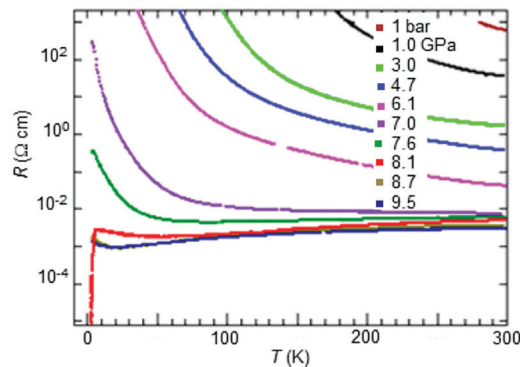
Fig. 8 Temperature dependence of electrical resistivity ( R ) of [\text{Ni}(\text{hfdt})_2] up to \sim 10 GPa. Adapted with permission from Cui, H., Kobayashi, H., Ishibashi, S., Sasa, M., Iwase, F., Kato, R., & Kobayashi, A. (2014). A Single-Component Molecular Superconductor. J. Am. Chem. Soc. , 136(21), 7619–7622. DOI: 10.1021/ja503690m. Copyright 2014 American Chemical Society.
