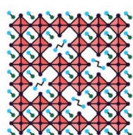
Hollow (3D)
