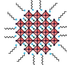
Nanocrystal (0D)
