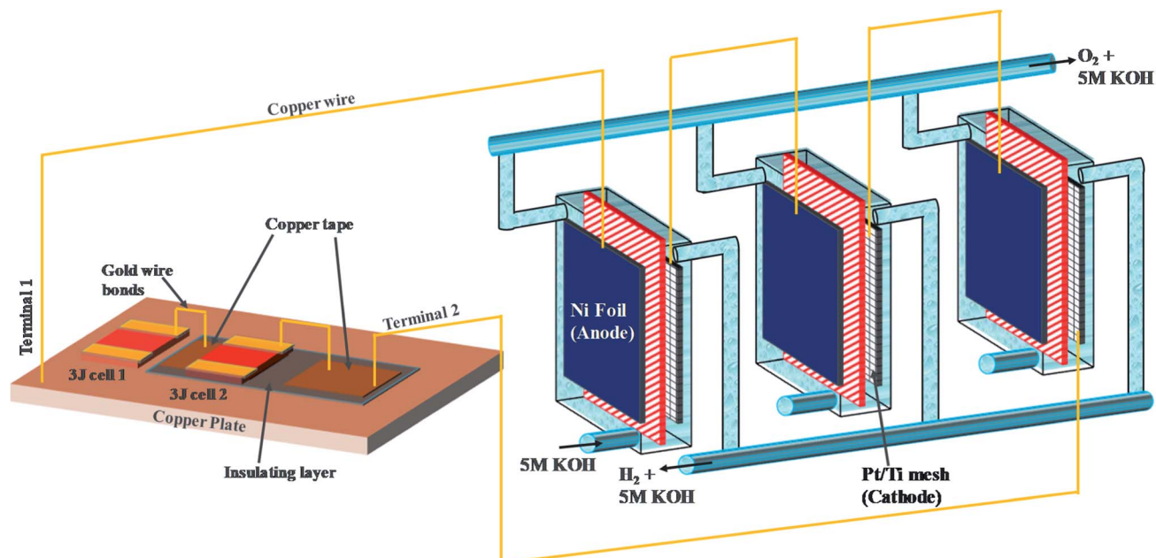
Scheme 1 The PV-electrolysis setup consists of two-3J CPV cells (each is composed of GaInP/GaInAs/Ge CPV cells ( 3.0 \times 3.0 mm 2 )) connected in series to three alkaline electrolyzers, also connected in series. Each alkaline electrolyzer is composed of ca. 10 nm Pt particles deposited on both sides of a Ti mesh (Pt/Ti mesh) as the cathode and a Ni(OH) 2 /Ni as the anode. The electrolyte (5 M KOH solution) is recirculated. Terminal 1: back side of the cells (+), and terminal 2: front side of the cell (–). Light at 41-sun concentration illuminated the cells, without the use of Fresnel lenses.
