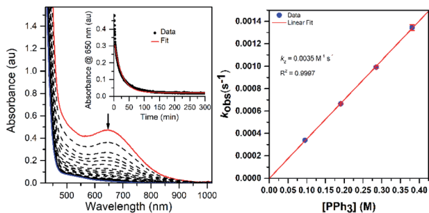
Fig. 10 Left: electronic absorption spectra monitoring the reaction of a 2.0 mM anaerobic solution of [\text{Mn}^{\text{III}}(\text{OO}^t\text{Bu})(^6\text{Me-dpaq})]^{+} (red trace) in \text{CH}_3\text{CN} with 100 equivalents of \text{PPh}_3 at 298 K. Left inset: time course for the spectral changes. Right: pseudo-first-order rate constants, k_{\text{obs}} ( \text{s}^{-1} ), versus \text{PPh}_3 concentration (M) for a 1.25 mM solution of [\text{Mn}^{\text{III}}(\text{OO}^t\text{Bu})(^6\text{Me-dpaq})]^{+} at 298 K.
