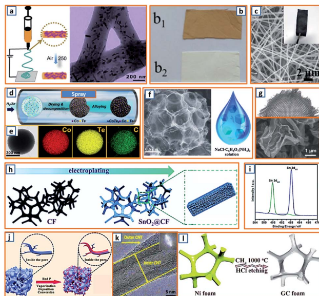
Fig. 8 Electrospinning, spray drying, electrodeposition, and CVD. (a) Electrospinning process and the corresponding microstructure of \text{Sb@CN} nanofibers. Reproduced with permission. 2 Copyright 2020, Elsevier. (b) As-spun preasphaltene/PAN (b1) and PAN (b2) fibers. Reproduced with permission. 27 Copyright 2020, American Chemical Society. (c) SEM images of \text{CuO/Cu-NCNFs} . Reproduced with permission. 46 Copyright 2020, Elsevier. (d) Schematic illustration of the spraying process and (e) corresponding elemental mapping of the \text{CoTe}_2\text{-C} composite. Reproduced with permission. 64 Copyright 2020, Elsevier. (f) SEM of the obtained N-doped interconnected carbon spheres and the \text{NaCl/C}_6\text{H}_{17}\text{N}_3\text{O}_7 precursor for spraying. Reproduced with permission. 81 Copyright 2019, The Royal Society of Chemistry. (g) Morphology of the activated crumpled graphene after the spray drying process. Reproduced with permission. 99 Copyright 2020, Wiley. (h) Schematic of the electrodeposition process of \text{SnO}_2\text{@CF} and (i) XRD spectrum after deposition. Reproduced with permission. 16 Copyright 2020, The Royal Society of Chemistry. (j) CVD for the fabrication of red \text{P@AC} . Reproduced with permission. 119 Copyright 2020, Elsevier. (k) Microstructure of multiwalled hierarchical carbon nanotube after CVD. Reproduced with permission. 125 Copyright 2018, Wiley. (l) CVD for the synthesis of graphitic carbon foam. Reproduced with permission. 129 Copyright 2019, The Royal Society of Chemistry.
