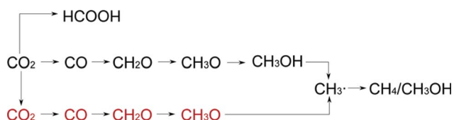
Fig. 6 Reaction pathway for the photocatalytic \text{CO}_2 conversion (red and black color font indicate the species adsorbed at the oxygen vacancy and on surface Ti, respectively) (reproduced from ref. 48 with permission from the American Chemical Society, copyright 2016).
