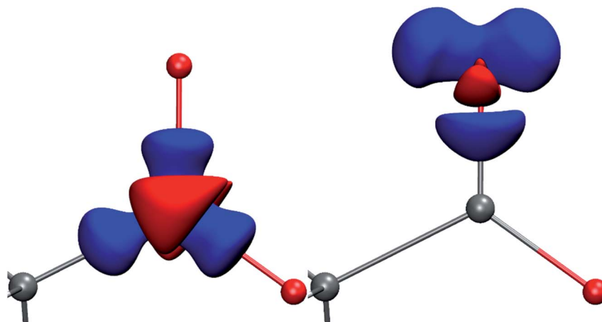
Fig. 1 Deformation Hirshfeld densities 12 for the carbon (left) and oxygen (right) atoms in the carboxylate group of Gly-L-Ala, i.e. difference between the spherical atomic electron density used in the IAM and the non-spherical Hirshfeld atom density used in HAR (IAM minus HAR). Red = negative, blue = positive. Isovalue = 0.17 \text{ e}\text{\AA}^{-3} .
