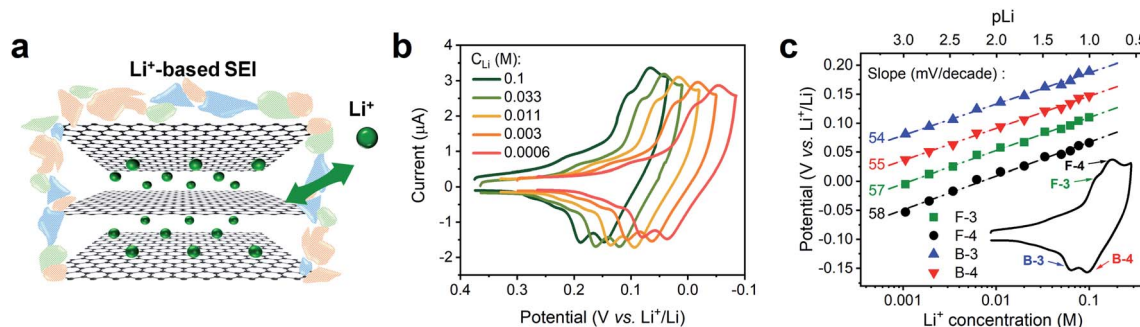
Fig. 2 Voltammetric characterization of Li + intercalation on FLG at various concentrations. (a) Depiction of Li + intercalation process in FLG with a Li + -based SEI. (b) Comparison of Li + intercalation CVs at selected Li + concentration ( C_{Li} ). (c) Relationship of Li + intercalation peak potential and C_{Li} at logarithmic scale (pLi) in panel (b) with labeled Nernstian-slopes, the inset CV indicates the selected peaks, F = forward/intercalation & B = backward/deintercalation. Li + intercalations at various C_{Li} were tested by spiking different amount of 0.1 M TBAPF 6 into 0.1 M LiPF 6 PC-EC solution, on 7.1 mm 2 FLG working electrode at 1 mV s -1 .
