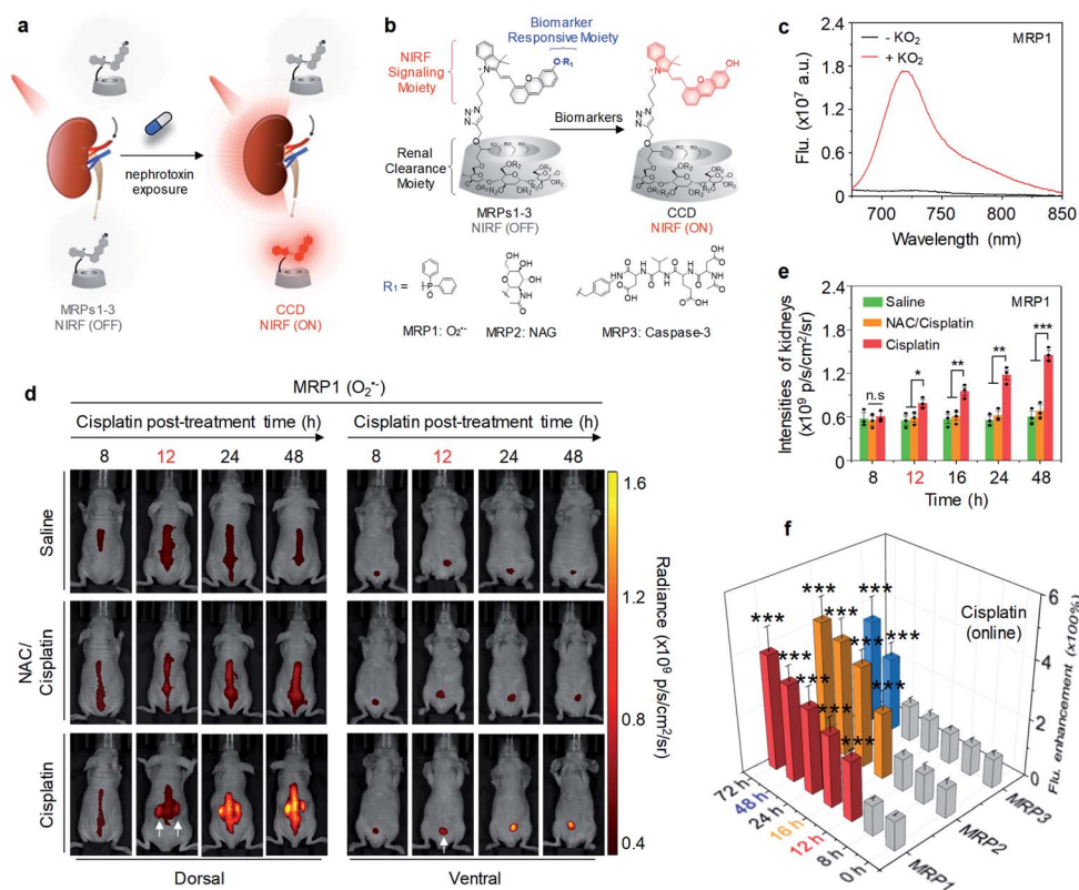
Fig. 5 (a) Schematic illustration of drug-induced AKI using MRPs1–3 . (b) Chemical structures and molecular mechanisms of MRPs1–3 and their activated forms in response to O_2^{\cdot-} , NAG and caspase-3, respectively, ( R = H or CH_2CHOHCH_3 ). (c) Fluorescence spectra of MRP1 (30 \mu M ) in the absence or presence of KO_2 (60 \mu M ) in PBS buffer (10 mM, pH 7.4). (d) Representative NIR fluorescence images of living mice with injection of MRP1 after treatment of cisplatin (20 mg per kg body weight) for 8, 12, 24 or 48 h. The control groups were treated with PBS or a nephroprotective antioxidant NAC. NIRF images acquired at 720 nm upon excitation at 675 nm. (e) NIRF intensities of kidneys in living mice after 30 min injection of MRP1 at the different post-treatment time points (8, 12, 16, 24 or 48 h). (f) Fluorescence enhancement of excreted MRPs1–3 in the urine from cisplatin-treated living mice after injection at different time points post-treatment of cisplatin. n.s.: not significant, *p < 0.05 , **p < 0.01 , ***p < 0.001 . Reproduced with permission from ref. 56. Copyright 2019 Springer Nature.
