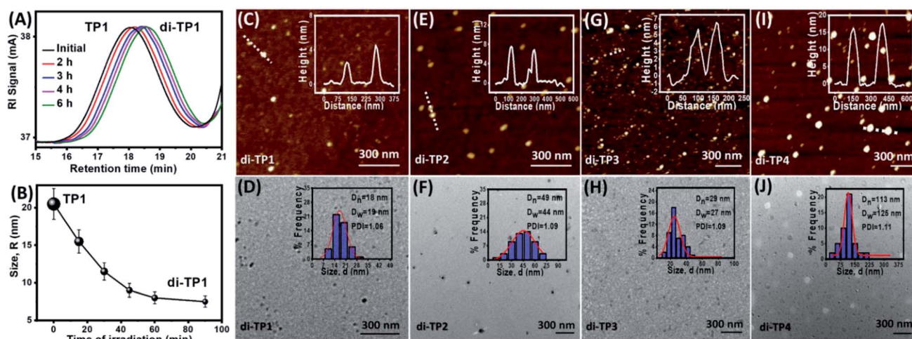
Fig. 3 (A) SEC analyses showing a delay in retention volume upon UV B irradiation of polymer sample TP1 (irradiation of sample solution ( c = 6 mg mL −1 in THF with 1 × 8 W UV B lamp, 6 h) (B) DLS data showing hydrodynamic radii ( R_H ) for the polymer TP1 upon irradiation (irradiation of sample solution, c = 10^{-3} mg mL −1 in 0.4 v/v% DMF–THF with 1 × 8 W UV B lamp, 8 h). AFM and TEM images of irradiated samples and their corresponding histogram analyses from (C and D) di-TP1, (E and F) di-TP2, (G and H) di-TP3, (I and J) di-TP4.
