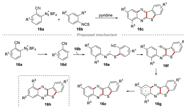
Scheme 16 The construction of benzothienoquinoxalines.
