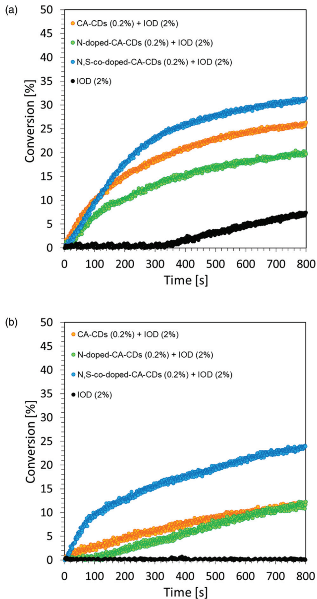
Fig. 10 Free-radical photopolymerization profiles (acrylate function conversion vs. irradiation time) for TMPTA with the bimolecular photoinitiating system based on IOD (2.0 wt%) and CA-CDs (0.2 wt%) (a) under irradiation at 365 nm; (b) under irradiation at 405 nm. Irradiance was measured at a distance of 210 mm for all sources.
