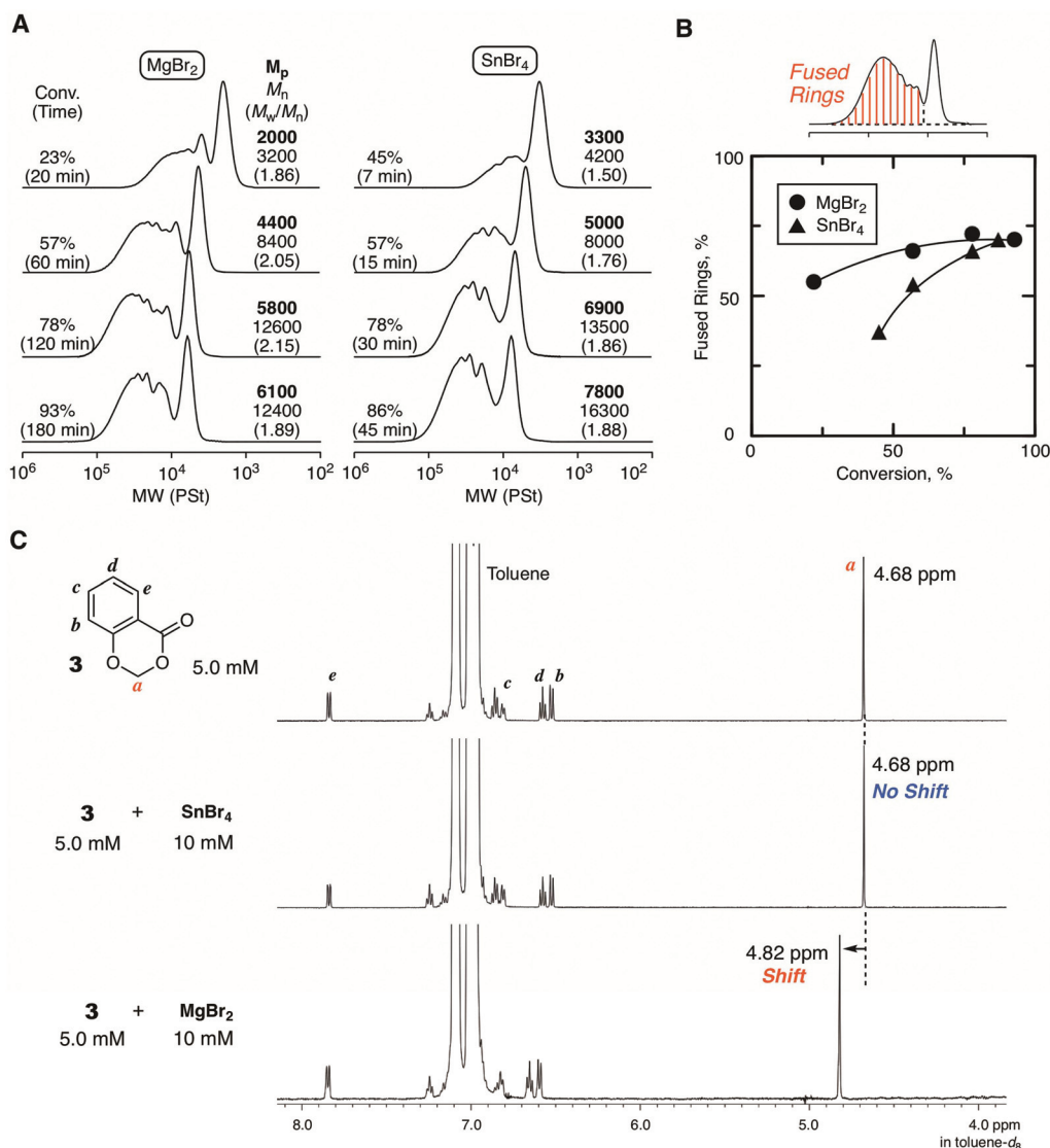
Fig. 4 Comparison between MgBr_2 and SnBr_4 in the ring-expansion cationic polymerization of IBVE with 1 : (A) SEC curves of the obtained poly (1BVE)s (B) ratios of the fused ring estimated by peak separation. (C) ^1H NMR analyses of the mixture of MgBr_2 or SnBr_4 with 3 as the model compound for the evaluation of the interaction with the HAE bond.
