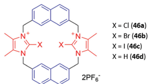
Fig. 24 Structures of proto- or halo-imidazolium-containing cyclophanes ( 46a-d ) with imidazolium shown in red and naphthalene fluorophores in blue. 46b bound \text{I}^- with K_a = 6.31 \times 10^5 \text{ M}^{-1} and 46d bound \text{Br}^- with K_a = 9.55 \times 10^5 \text{ M}^{-1} in 9 : 1 \text{CH}_3\text{OH}/\text{H}_2\text{O} .
