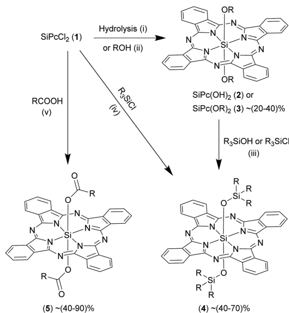
Scheme 4 Reactions of SiPcCl 2 , ( 1 ) where axial chlorides are replaced by alcohols, phenols, silanes and carboxylic acids. Reagents and conditions: (i) NaOCH 3 , 95% CH 3 CH 2 OH, reflux, 1 h; (ii) ROH, toluene, pyridine or sodium hydride, reflux, 120 °C, 24–96 h; (iii) R 3 SiOH or R 3 SiCl, toluene, pyridine, reflux, 120 °C, 3–6 h; (iv) R 3 SiCl, NaOH, Aliquat HTA-1, chlorobenzene, reflux, 132 °C; (v) RCOOH, methoxyethyl ether, reflux, 160 °C, 0.5–6 h. R represent aryl or alkyl groups.
