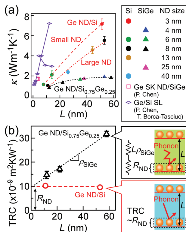
Fig. 3 The L dependence of (a) \kappa and (b) TRC. In (a), the red dashed and the red dotted lines are the eye-guides for the Ge ND/Si films with the small and the large Ge ND sizes, respectively. The black dotted line is the eye-guide for the Ge ND/ \text{Si}_{0.75}\text{Ge}_{0.25} films. In (b), the black dotted line for the Ge ND (8 nm)/ \text{Si}_{0.75}\text{Ge}_{0.25} film is the line-fitted curve with eqn (1) and the red dashed line for the Ge ND (8 nm)/Si film shows no dependence of TRC on the L . R_{\text{ND}} values for the Ge ND/Si films are roughly consistent with those of our previous study. 13 In the right side of (b), the schematics of one cycle structures, and the thermal circuit model of the Ge ND/SiGe films: \text{TRC} = L\rho_{\text{SiGe}} + R_{\text{ND}} .
