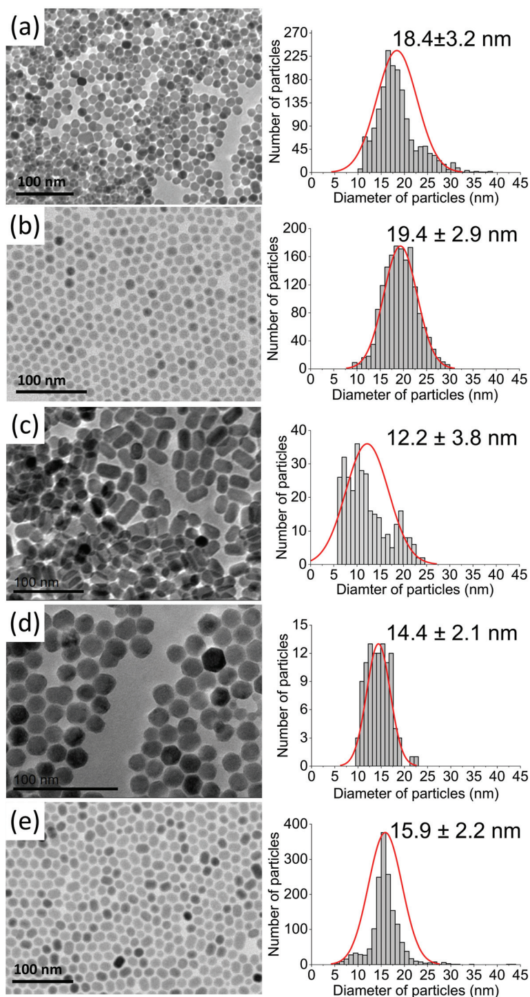
Fig. 2 TEM images recorded for (a) \text{NaYF}_4:2\%\text{Tm}^{3+}@ \text{NaYF}_4 , (b) \text{NaYF}_4:2\%\text{Tm}^{3+},5\%\text{Er}^{3+}@ \text{NaYF}_4 , (c) \text{NaYF}_4:2\%\text{Tm}^{3+}@ \text{NaYF}_4:5\%\text{Er}^{3+} , (d) \text{NaYF}_4:18\%\text{Yb}^{3+},2\%\text{Tm}^{3+}@ \text{NaYF}_4 , and (e) \text{NaYF}_4:18\%\text{Yb}^{3+},2\%\text{Tm}^{3+}@ \text{NaYF}_4:5\%\text{Er}^{3+} NPs.
