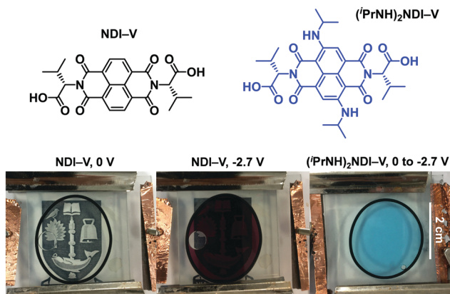
Fig. 1 The chemical structures of NDI-V and (\text{PrNH})_2\text{NDI-V} along with a display of the electrochromic properties of NDI-V and the lack of electrochromic properties of (\text{PrNH})_2\text{NDI-V} . Both species were dissolved in water with 40% v/v 0.1 M NaCl electrolyte at pH 8.
