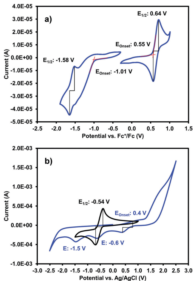
Fig. 2 (a) The cyclic voltammogram for (\text{PrNH})_2\text{NDI-V} measured in DCM with 0.1 M \text{NBu}_4\text{PF}_6 electrolyte. Oxidation and reduction onsets and E_{1/2} potentials are shown. (b) The cyclic voltammograms for (\text{PrNH})_2\text{NDI-V} (blue trace) and NDI-V (black trace) measured in water with a 40% v/v 0.1 M NaCl electrolyte at pH 8.
