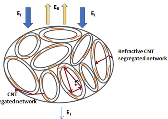
Fig. 14 Schematic illustration of the EMI shielding mechanisms for the segregated network of PE/CNT composites (modified from ref. 208 with permission from MDPI, copyright 2020).
