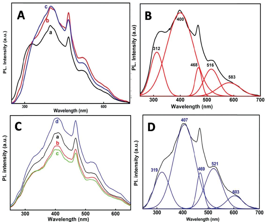
Fig. 7 (A) Room temperature PL spectra of tin oxide nanoparticles synthesized at different temperatures in relin ( \lambda_{exc} = 220 nm), (a) 50 °C; (b) 80 °C; and (c) 98 °C. (B) De-convoluted fitting plot of the PL spectrum of the nanoparticles obtained at 50 °C with \lambda_{exc} = 220 nm. (C) Room temperature PL spectra of tin oxide nanoparticles synthesized at different e-beam irradiation doses in the relin host matrix ( \lambda_{exc} = 220 nm), (a) 35 kGy; (b) 72 kGy; (c) 107 kGy and (d) 143 kGy. (D) De-convoluted fitting plot of the PL spectrum of the nanoparticles (by the e-beam irradiation method) at \lambda_{exc} = 220 nm.
