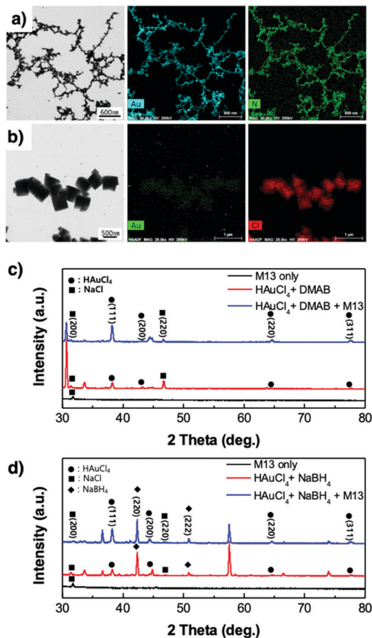
Fig. 3 STEM images and EDS analysis of the virus-templated Au nanowires formed under (a) DMAB and (b) NaBH 4 . XRD spectra of the virus-templated Au nanowires formed under (c) DMAB and (d) NaBH 4 .
