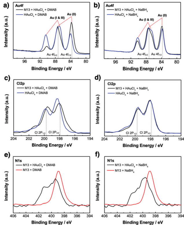
Fig. 4 XPS measurements of Au 4f peaks of the virus-templated Au nanowires made under (a) DMAB or (b) NaBH 4 (blue). (c) Cl 2p peaks of the virus-templated Au nanowires made under (c) DMAB or (d) NaBH 4 . N 1s peaks of the virus-templated Au nanowires made under (e) DMAB and (f) NaBH 4 .
