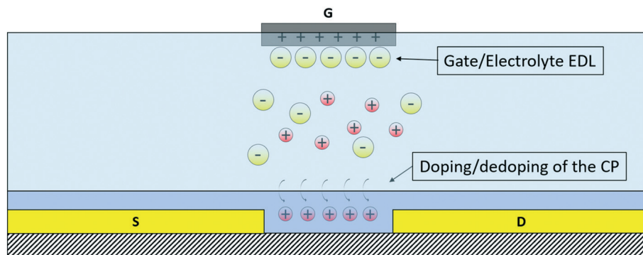
Fig. 2 The OEFT working principle. The channel current I_D is modulated by the application of a gate voltage, which promotes the doping/dedoping of the CP layer. Since the whole volume of the CP layer is affected by the doping/dedoping mechanism, this device is characterized by a volumetric capacitance that helps to obtain high transconductances, and thus high sensitivities and low operating voltages. The doping/dedoping mechanism can be influenced by the presence of a cell layer on the surface of the CP.
