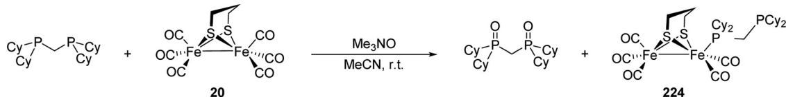
Fig. 66 Reaction of dcmp with complex 20 in the presence of \text{Me}_3\text{NO} .
