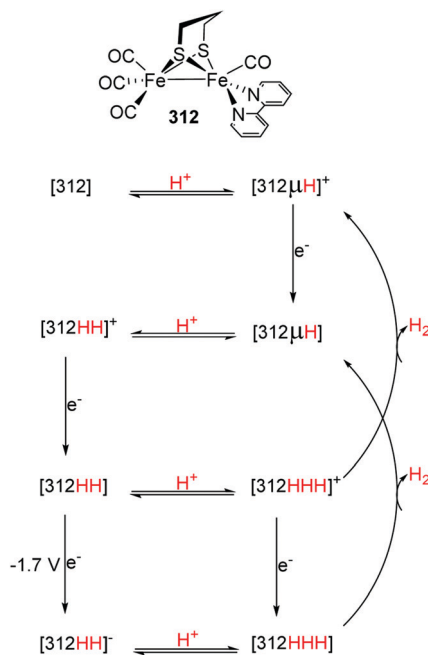
Fig. 104 Catalytic pathway for HER from HBF 4 ·OEt 2 by 312 . 371
