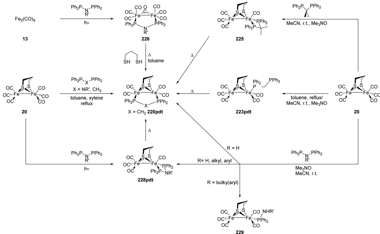
Fig. 65 Different synthetic pathways for the incorporation of dpmm and derived ligands as well as PNP ligands into hydrogenase mimics.
