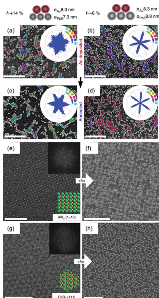
Fig. 3 (a–d) SEM images and bond angle plots of Au nanoparticles assembled on PbS nanoparticle monolayers before (a and b) and after (c and d) solvent annealing at different lattice misfits. (e) SEM image of the \text{AlB}_2 structure assembled from 15.5 nm \text{Fe}_3\text{O}_4 and 8.3 nm Au nanoparticles. (f) SEM image of the epitaxial assembly formed by the deposition of 8.3 nm Au nanoparticles on the structure in (e). (g) SEM image of the 111 projection of the \text{CaB}_6 structure assembled from 15.5 nm \text{Fe}_3\text{O}_4 and 6.0 nm Au nanoparticles. (h) SEM image of the epitaxial assembly formed by the deposition of 8.3 nm Au nanoparticles on the structure in (g). Upper insets in (e and g) are fast Fourier transform (FFT) patterns of the images. Lower insets in (e and g) are models of the lattice projections. All scale bars are 100 nm. 33
