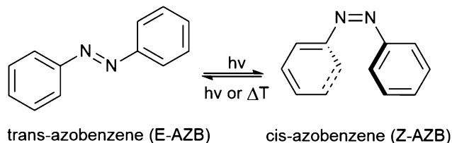
Scheme 1 Azobenzene trans \rightleftharpoons cis isomerisation.
