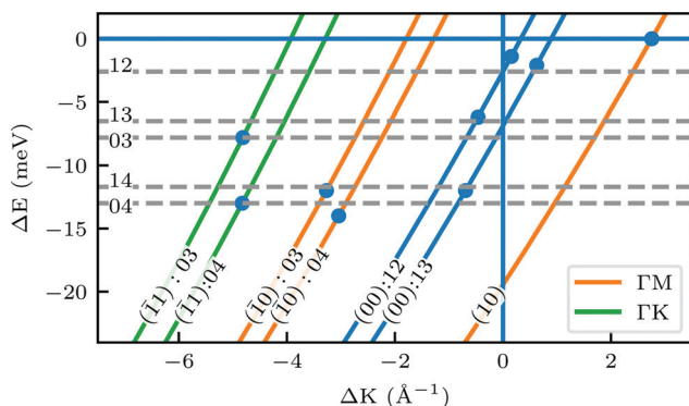
Fig. 2 Maximum energy loss values from the TOF spectra plotted on their corresponding scan curves and compared to the rotational transition energies of CH 4 (gray dashed lines). Scan curve labels indicate the corresponding RID peak from Fig. 1A and B. Scan curves are plotted in orange, green and blue if they correspond to \overline{\Gamma M} , \overline{\Gamma K} or both directions, respectively.
