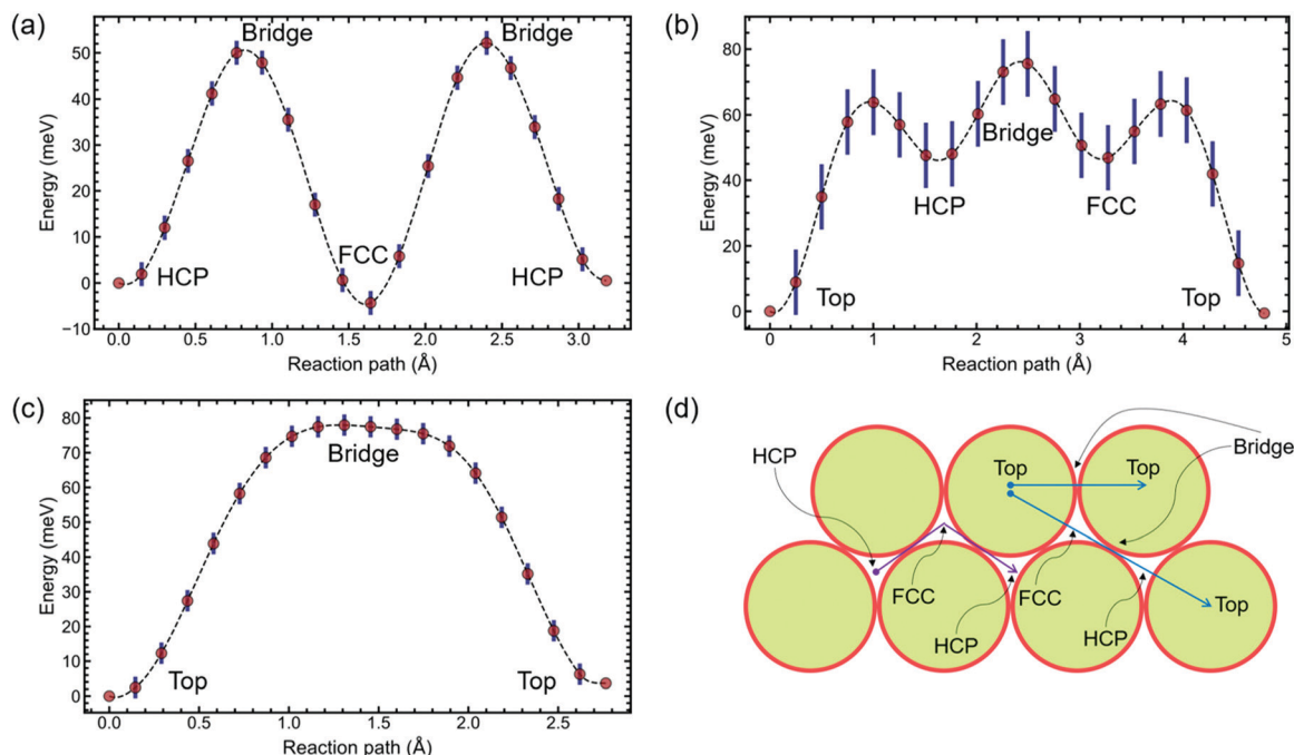
Fig. 3 DFT-calculated potential energy landscapes. Blue and Magenta arrows Panel (d) show the relevant diffusion paths. (a) Na(2 × 2)/Ru(0001) hallow-to-hollow jump diffusion with the bridge site as the transition state. Note that the FCC and HCP sites are degenerate within the accuracy of the calculation. (b) and (c) Na(4 × 4)/Ru(0001) top-to-top jump diffusion (b) via local minima hollow sites to a second-nearest neighbour, and (c) to the nearest neighbour, directly across a bridge site. As in the 2 × 2 calculation, the FCC and HCP sites are nearly degenerate in the 4 × 4 calculation (not shown explicitly).
