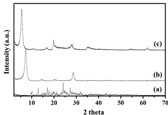
Fig. 2 Powder X-ray diffraction patterns of (a) BMD, (b) pristine MMT, and (c) BMD–MMT.
