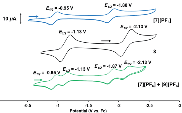
Fig. 7 Cyclic voltammograms (in 0.3 M [t\text{Bu}_4\text{N}][\text{PF}_6] in THF; scan rate: 100\text{ mV s}^{-1} ) of compounds [7][\text{PF}_6] (blue), 8 (black), and a mixture of [7][\text{PF}_6] and [9][\text{PF}_6] obtained from the reaction of 8 with \text{FcPF}_6 (green).
