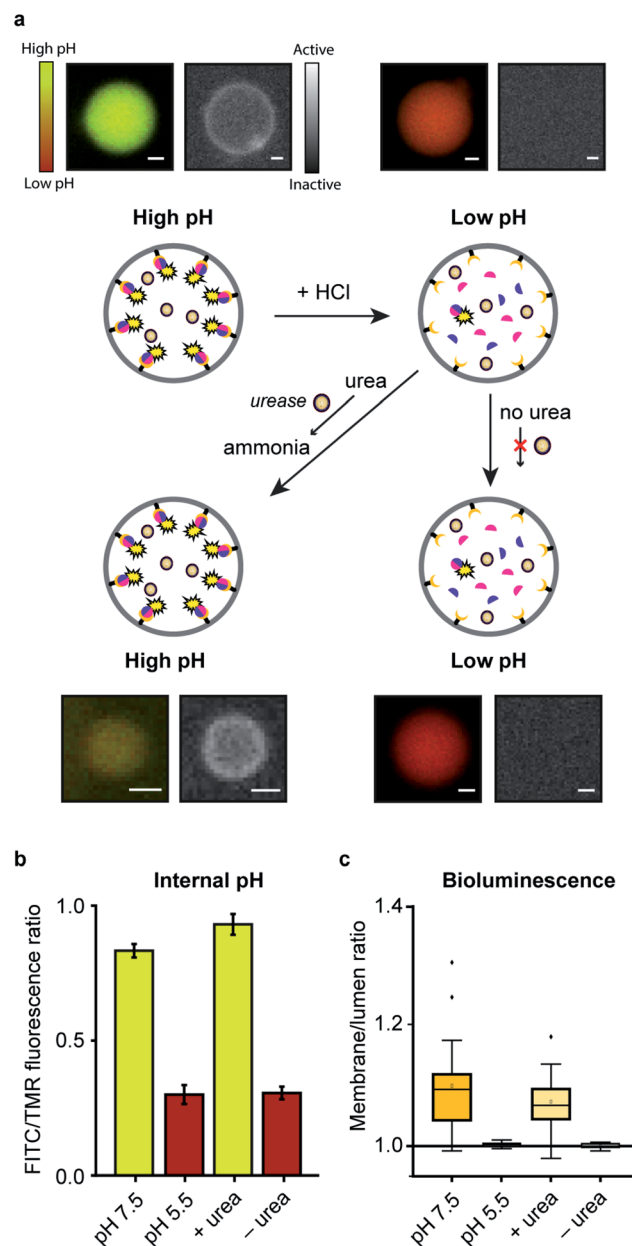
Fig. 4 Integrated pre-programmed control over spatio-structural organization and enzymatic signaling in GUVs. (a) Spatial-structural organization and enzymatic signaling of LgBiT and SmBiT ( 5 \mu\text{M} each) is promoted at pH 7.5. Addition of HCl dissociated the complex. Next, urea served as an environmental cue to restore enzymatic signaling at the membrane. Fluorescence micrographs of representative GUVs display internal pH (left panels) and bioluminescence micrographs indicate enzymatic signaling (right panels). Scale bars represent 5 \mu\text{m} . (b) The internal pH of >40 GUVs was tracked using a fluorescent ratiometric pH probe (dextran-FITC-TMR). (c) The bioluminescence localization was quantified by comparing the integrated signal at the membrane and inside the lumen ( n_{\text{GUVs}} = 18 ).
