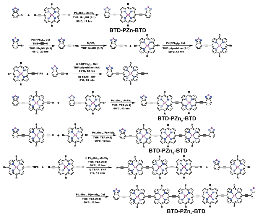
Scheme 2 Synthetic routes for BTD-PZn n -BTD compounds.
