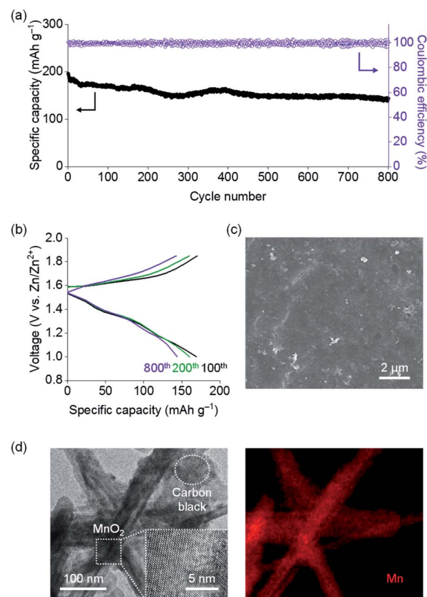
Fig. 4 (a) Cycling performance of a Zn|TpPa- \text{SO}_3\text{Zn}_{0.5} -| \text{MnO}_2 cell. (b) Charge/discharge profiles at the 100 th , 200 th and 800 th cycles. (c) SEM image of the Zn metal anode after the 800 th cycle. (d) TEM (left) and EDS mapping (for Mn; right) images of the \text{MnO}_2 cathode after the 800 th cycle.
