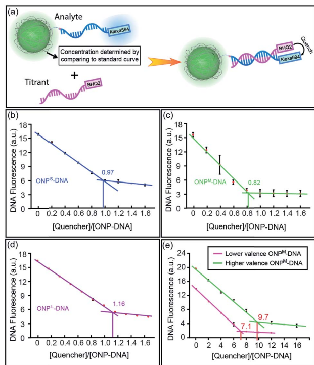
Fig. 4 (a) Cartoon illustration of the fluorescence titration experiment determining the ratio of DNA/ONP on different DNA-ONP conjugates. (b–d) Fluorescence titration results of DNA-ONP S/M/L -DNA. (e) Fluorescence titration results of the two polyvalent DNA-ONP M conjugates.
