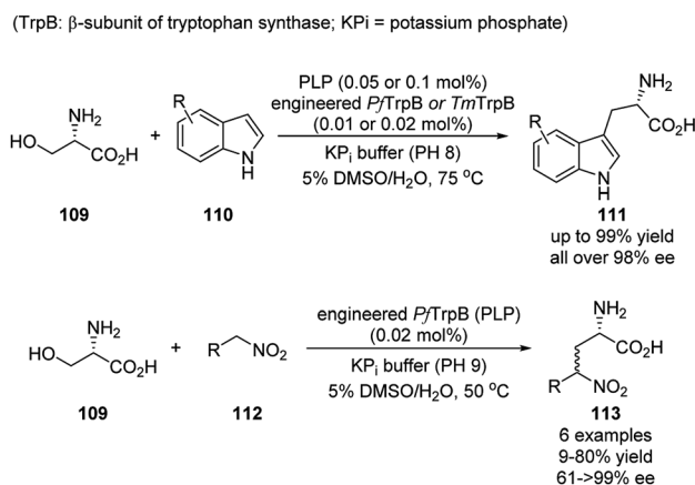
Scheme 32 Engineered TrpB catalyzed elimination/Micheal addition sequence.
