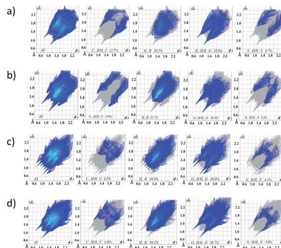
Fig. 9 The full two-dimensional fingerprint plot and fingerprint plots delineated into \text{C}\cdots\text{H}/\text{H}\cdots\text{C} , \text{H}\cdots\text{H} , \text{O}\cdots\text{H}/\text{H}\cdots\text{O} and \text{N}\cdots\text{H}/\text{H}\cdots\text{N} contacts for \text{H}_2\text{L} (a), \text{NaHL}\cdot\text{i-PrOH} (b), [\text{Tb}(\text{HL})_2(\text{NO}_3)]\cdot\text{i-PrOH} (c), [\text{Eu}(\text{HL})_2(\text{NO}_3)]\cdot\text{i-PrOH} (d).
