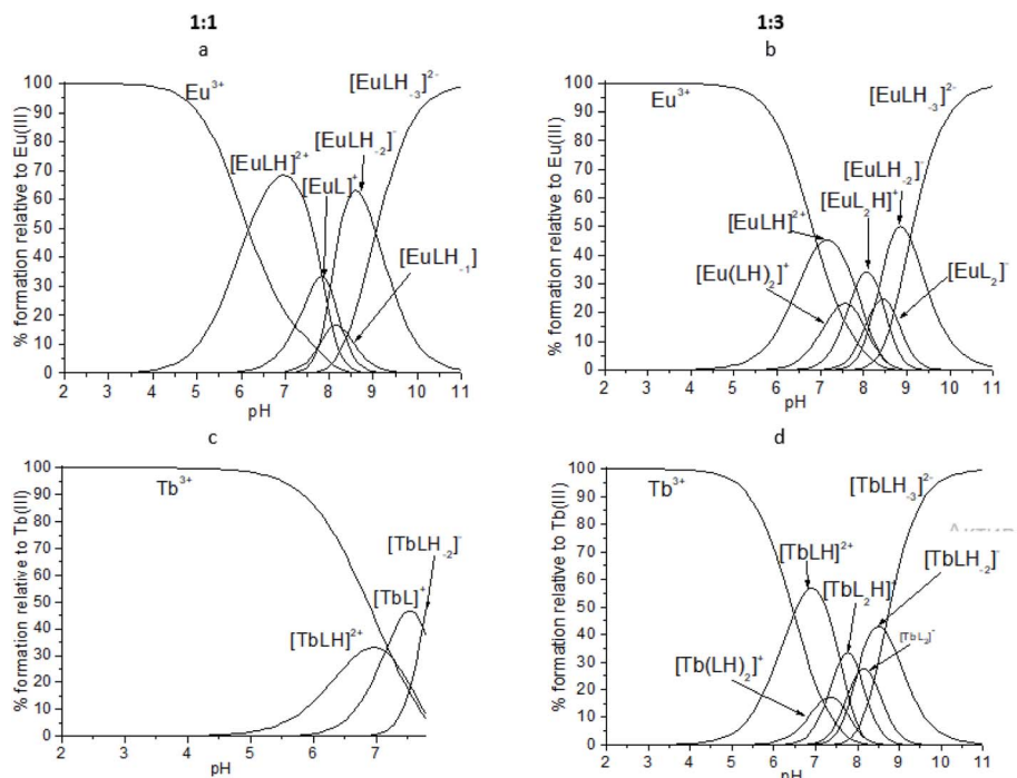
Fig. 12 Representative distribution diagrams for the systems \text{Eu}^{3+} (a and b) \text{H}_2\text{L} and \text{Tb}^{3+} (c and d) \text{H}_2\text{L} . Metal-to-ligand ratio of 1 : 1 and 1 : 3, [\text{L}] = 2 \text{ mM} , I = 0.1 \text{ M NaCl} .
